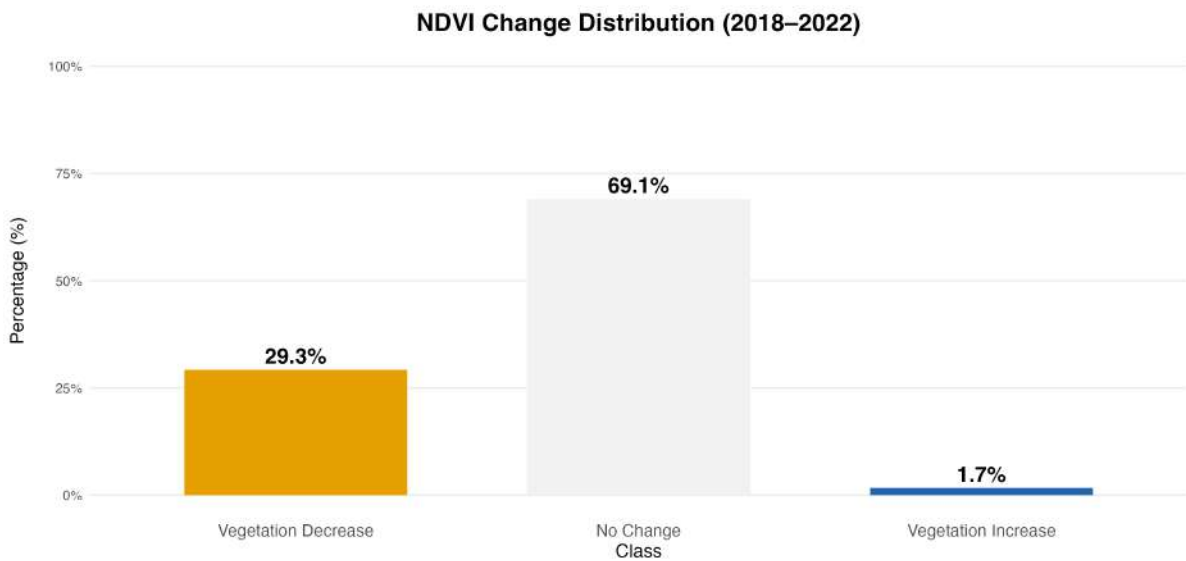
Figure 5.2: NDVI change map and NDVI change distribution in the Pra River Basin between 2018 and 2022.
